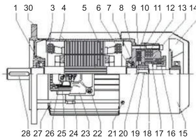
Figure 2 B5 63~112
