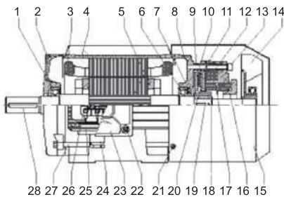
Figure 1 B3 63~160
