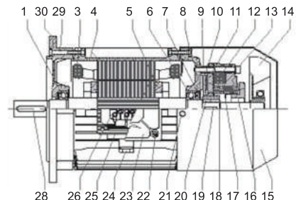
Figure 3 B5 132~160
