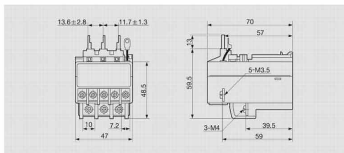
EOCR-SP / SP2-20Type
