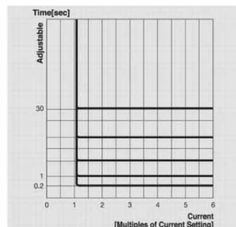
Curve-2 Definite
