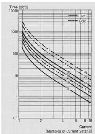
Curve-1 Inverse
