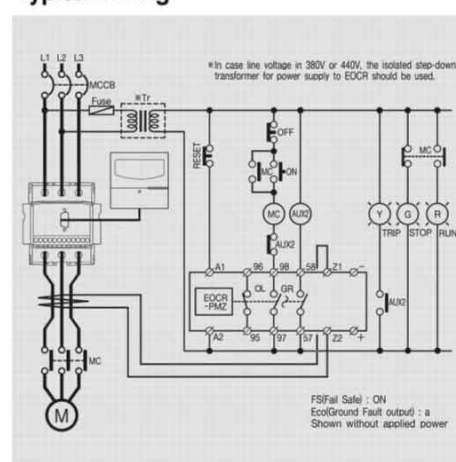
EOCR-PFZ (Terminal Type)
