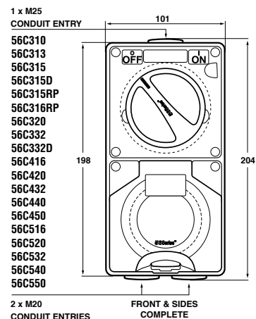
Dimensional Drawings
