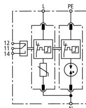
Basic circuit diagram VT2 M TT 2P 385 CN FM
