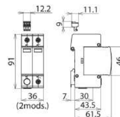
Dimension drawing VT2 M TT 2P 385 CN FM
