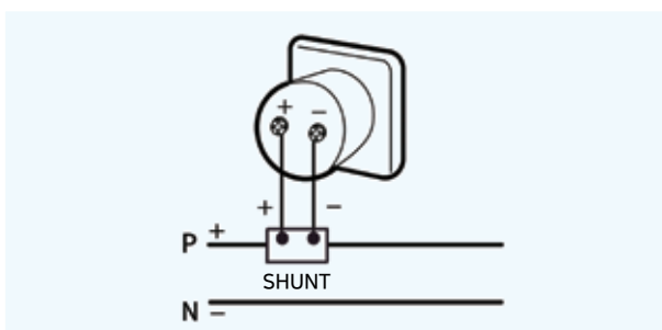
Shunt connection
