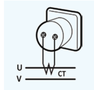
CT connection
