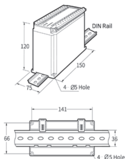
LL Type(Unit : mm)
