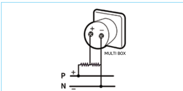
Voltage divider connection
