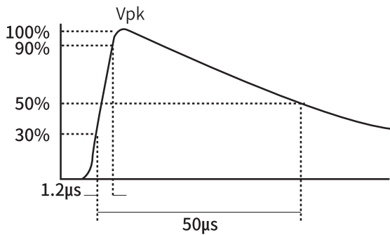
Voltage waveform
