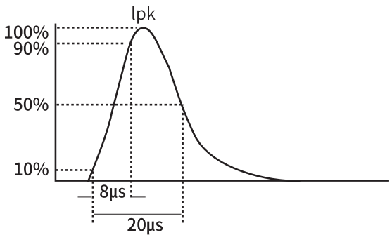
Current waveform
