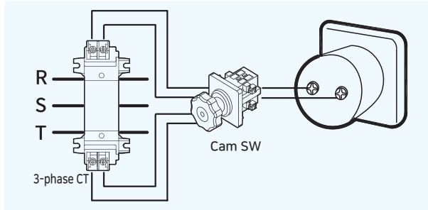
3P A/S connection
