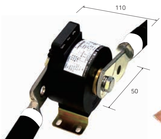
Single installation Type 1 H:120
