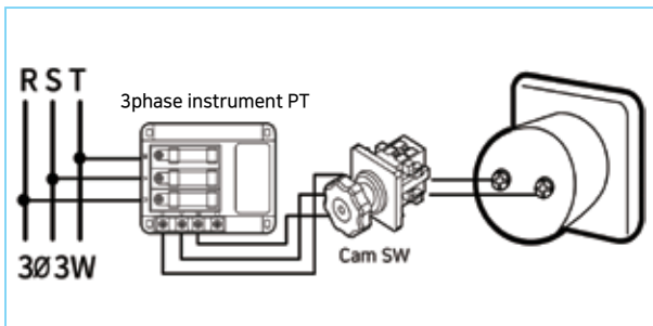
3P V/S connection
